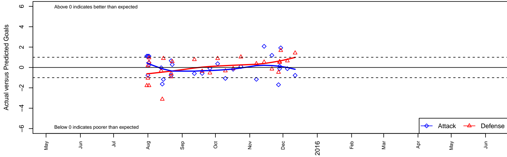
NSC Annihilation B01 Dots are actual minus expected GF (blue circles) and GA (red triangles). Blue line is smoothed change in attack strength. Red is smoothed change in defense strength.
